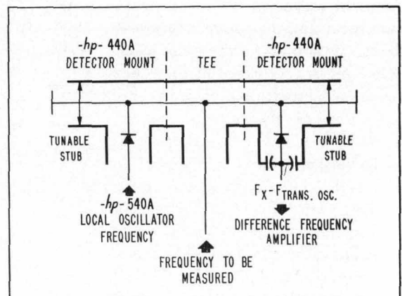
Fig. 10. Schematic arrangement of two -hp- Model 440A Detector Mounts as used to increase sensitivity of measurements in range above 5 kmc.
