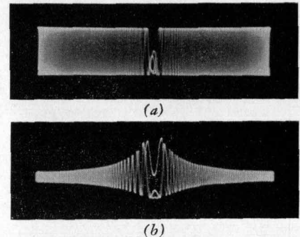
Fig. 6. Typical scope patterns obtained when (a) signal has wide excursions and (b) when excursions are so wide that display is limited by system bandwidth.
