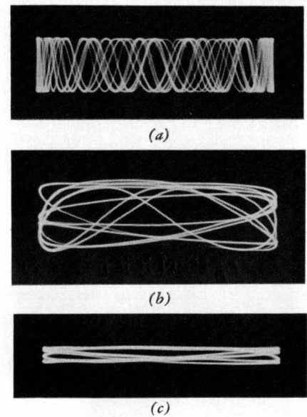
Fig. 3. Typical sequence of patterns obtained on transfer oscillator's scope as difference frequency is reduced to zero on a stable signal. Note that internal scope uses a 60-cycle sweep.
