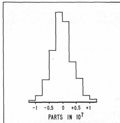
Fig. 7. Distribution of error of comparison in 250 measurements made by five operators.
