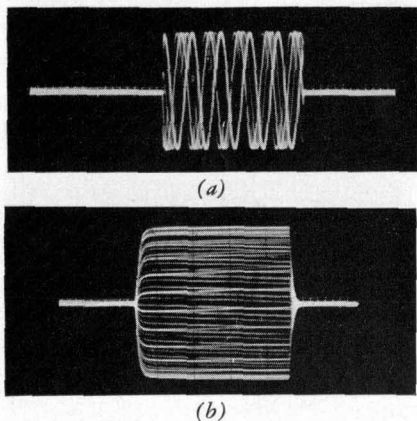
Fig. 8. Typical scope patterns obtained in pulsed r-f measurement as (a) zero beat is first approached and (b) when beat frequency has been made very small.
