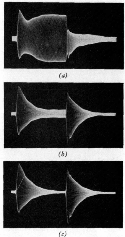
Fig. 9. Typical sequence of scope patterns obtained with sawtooth presentation as zero beat is approached (a) and (c) when beat frequency has been reduced to low value.
