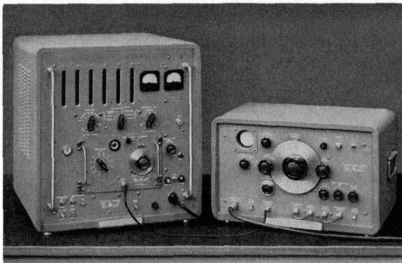
Fig. 1. New -hp- Model 540A Transfer Oscillator (right) operates with -hp- 524B High Speed Counter and 525B Converter to form precision measuring system capable of operation from 0 cps to 12,400 megacycles.
